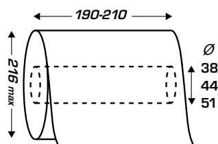
SIZES OF PAPER
