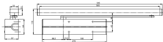
DCG460 guide rail
