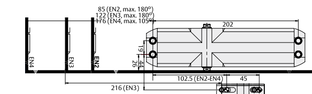
Transom mounting: Push side
