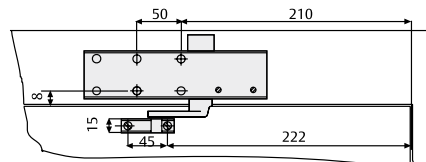
Mounting on push side
