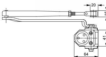
Mounting on pull side
