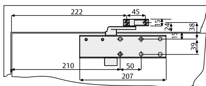
Mounting on pull side
