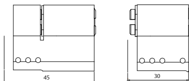
European modular heads (to be used with the modular cases)
