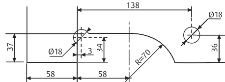
Glass machining
