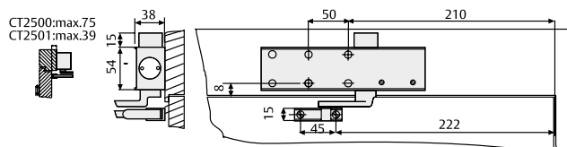
Mounting on push side
