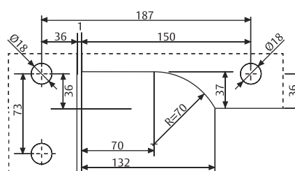
Glass machining
