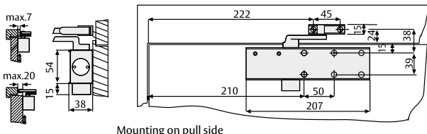
Mounting on pull side
