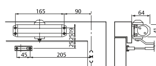
Mounting on push side
