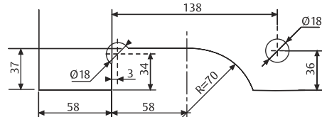
Glass machining
