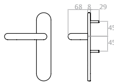
Lever handle
