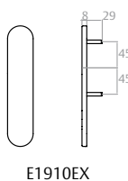
Blind plate
