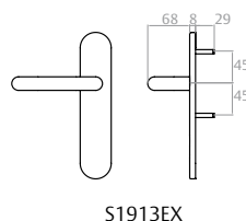
Lever handle
